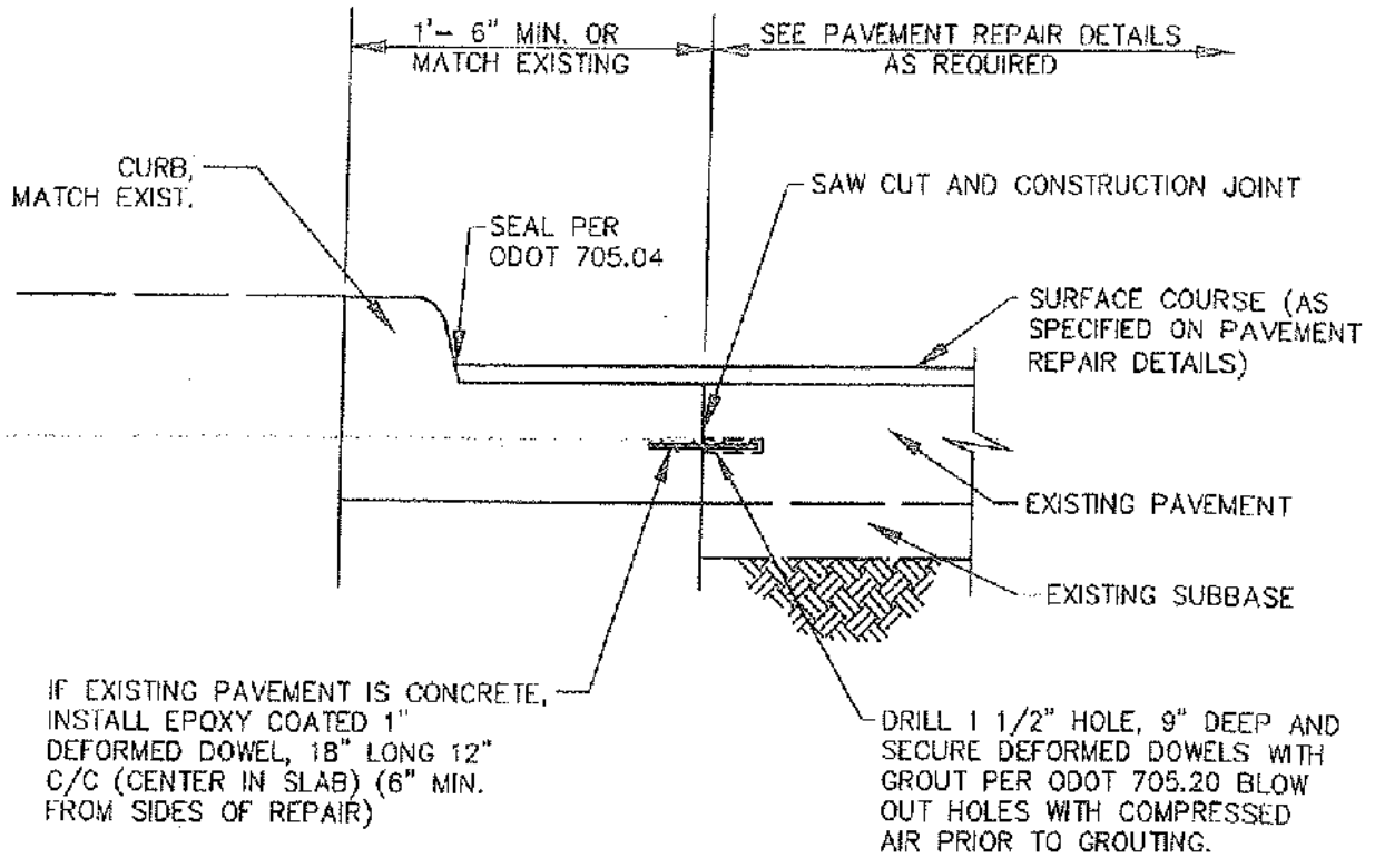
INTEGRAL CONCRETE CURB REPAIR DETAIL N.T.S.
